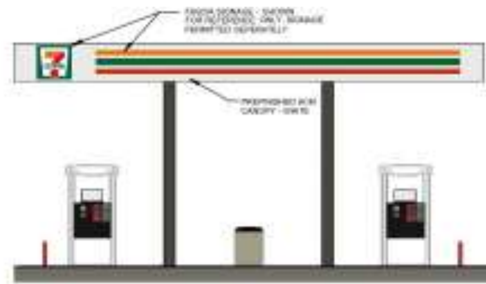
7 CANOPY ELEVATION - SHORT SIDE
