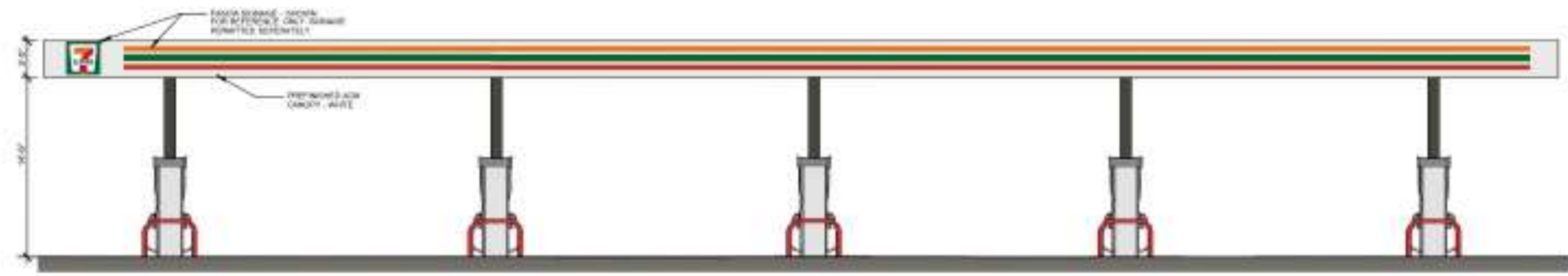
6 CANOPY ELEVATION - LONG SIDE
